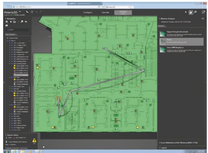
Analysis: View of route from the selected node back to the Wireless Manager (WM)
