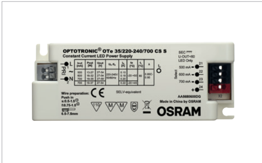
OPTOTRONIC® ECO driver (OTe 35/220-240/700 CS S)
